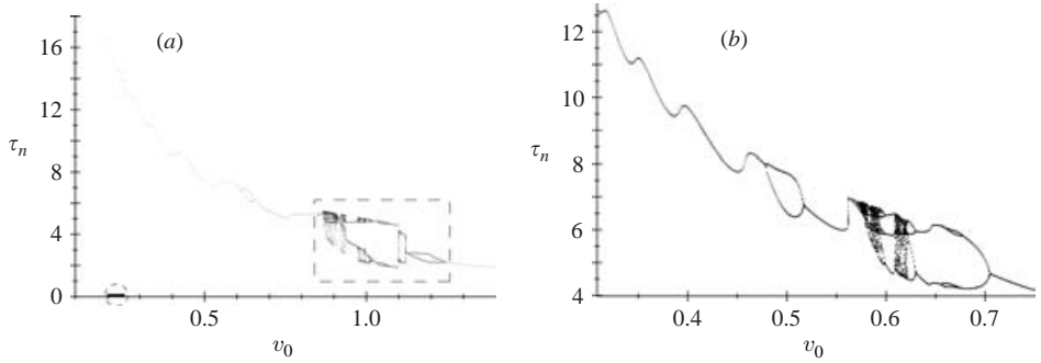
FIGURE 11. Bifurcation diagram derived from (a) the full hydrodynamic model (3.6) ( R=0.5 , \eta=0.02 , g=1 , \gamma=1 ), (b) the simple low-dimensional model (5.1), (5.2) ( \alpha=10 , \beta=0.028 , \gamma=-0.106 , \delta=-0.154 ). \tau_n corresponds to the time between two drops and v_0 is the exit velocity. The two bifurcation diagrams are qualitatively very similar.
