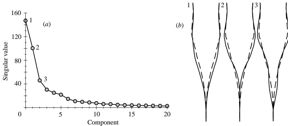
FIGURE 6. A proper orthogonal decomposition (POD) of the numerical simulation of the hydrodynamical equations (3.6) for the dripping faucet ( R=0.5 , \eta=0.02 and v_0=1.025 ). (a) Singular values are plotted for each ‘mode’. (b) The first three modes from the POD superposed on the average drop shape: 1 corresponds to V_1 + r_{av} , 2 corresponds to V_2 + r_{av} and 3 corresponds to V_3 + r_{av} (the dashed line corresponds to the interpolated average drop shape r_{av} ) computed as described in the text. Here V_i corresponds to the i th column of the matrix POD as indicated in the text. We see that just the first three modes capture much of the dynamical behaviour of the faucet.
